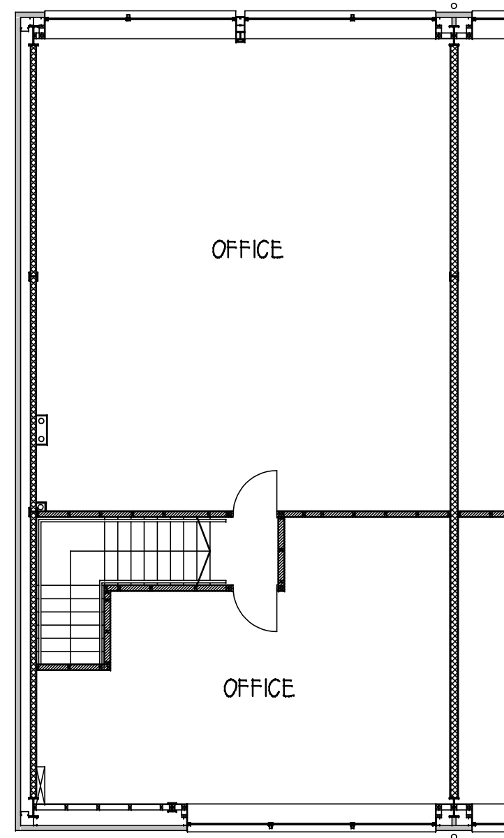
UNITS 6-9 FIRST FLOOR PLAN
