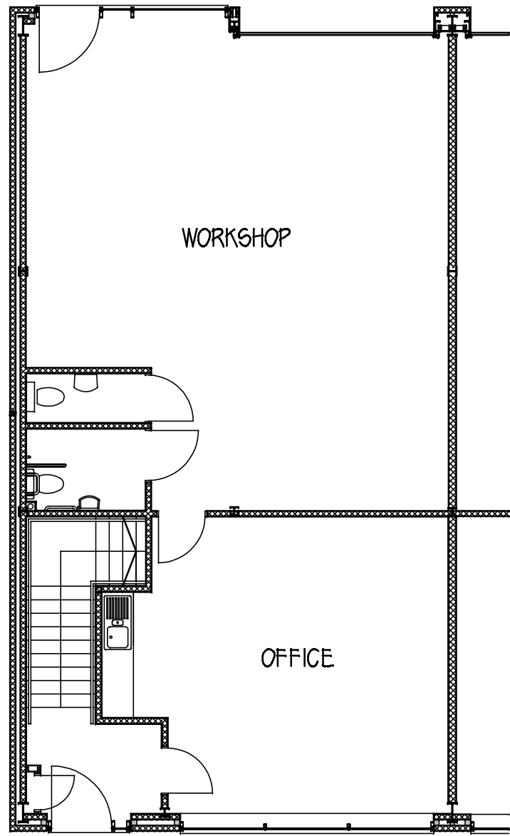
UNITS 6-9 GROUND FLOOR PLAN
