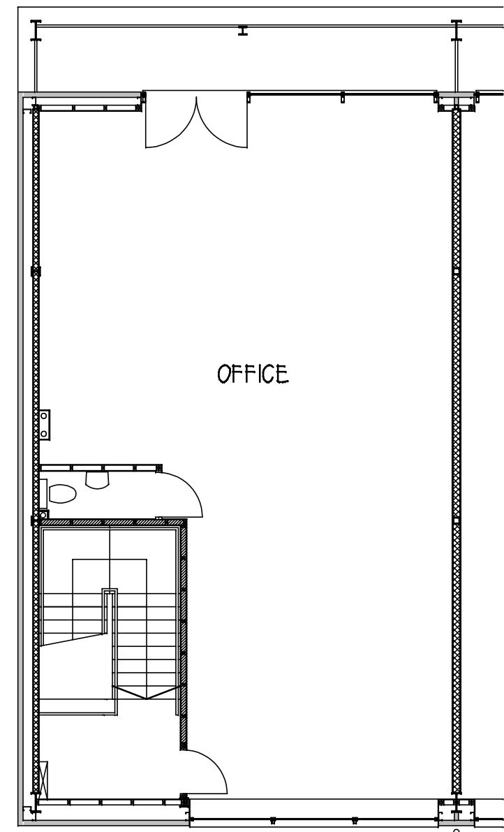
UNITS 10-13 SECOND FLOOR PLAN
